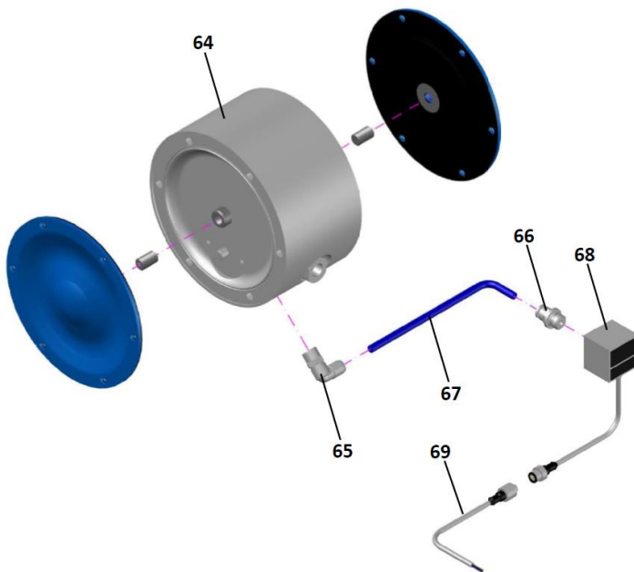
Spare part list, Stroke Counting Options: SC5, SC6 (pneumatic electronic sensor)
